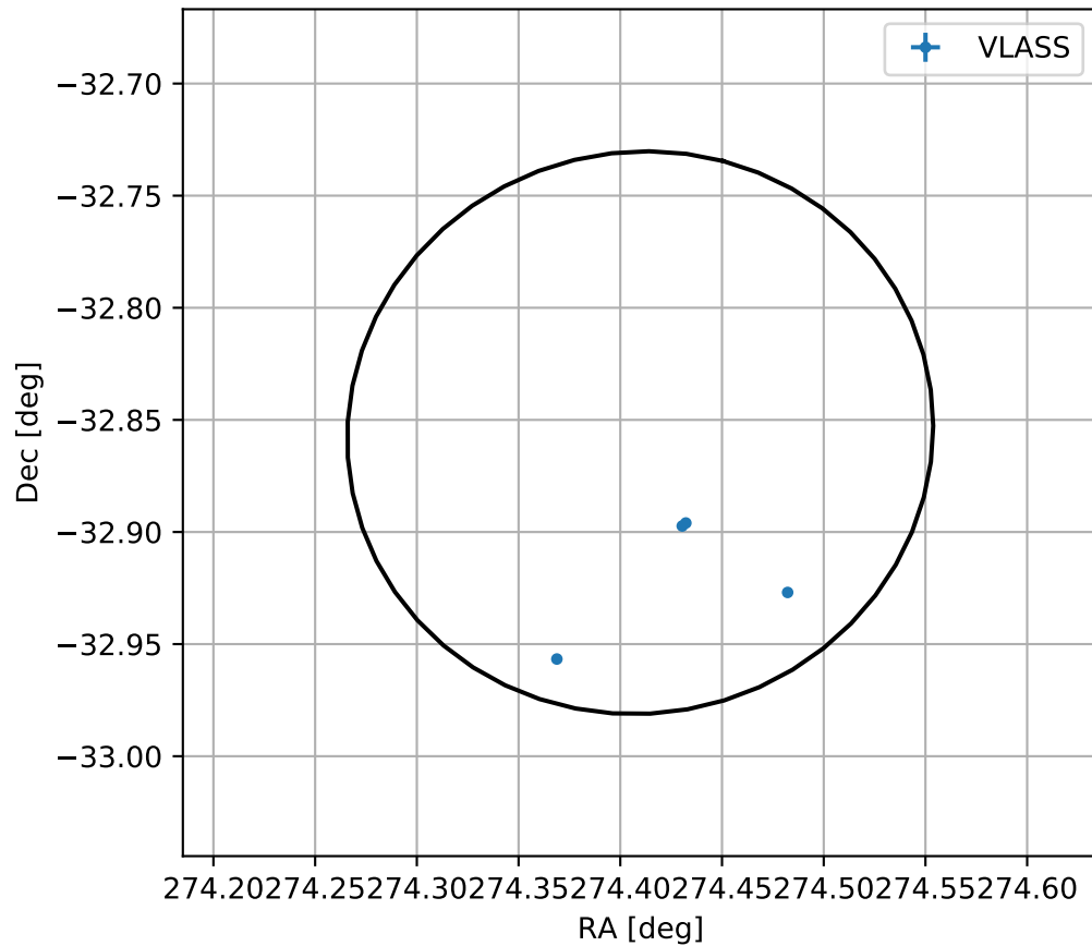
4FGL J1817.6-3251
