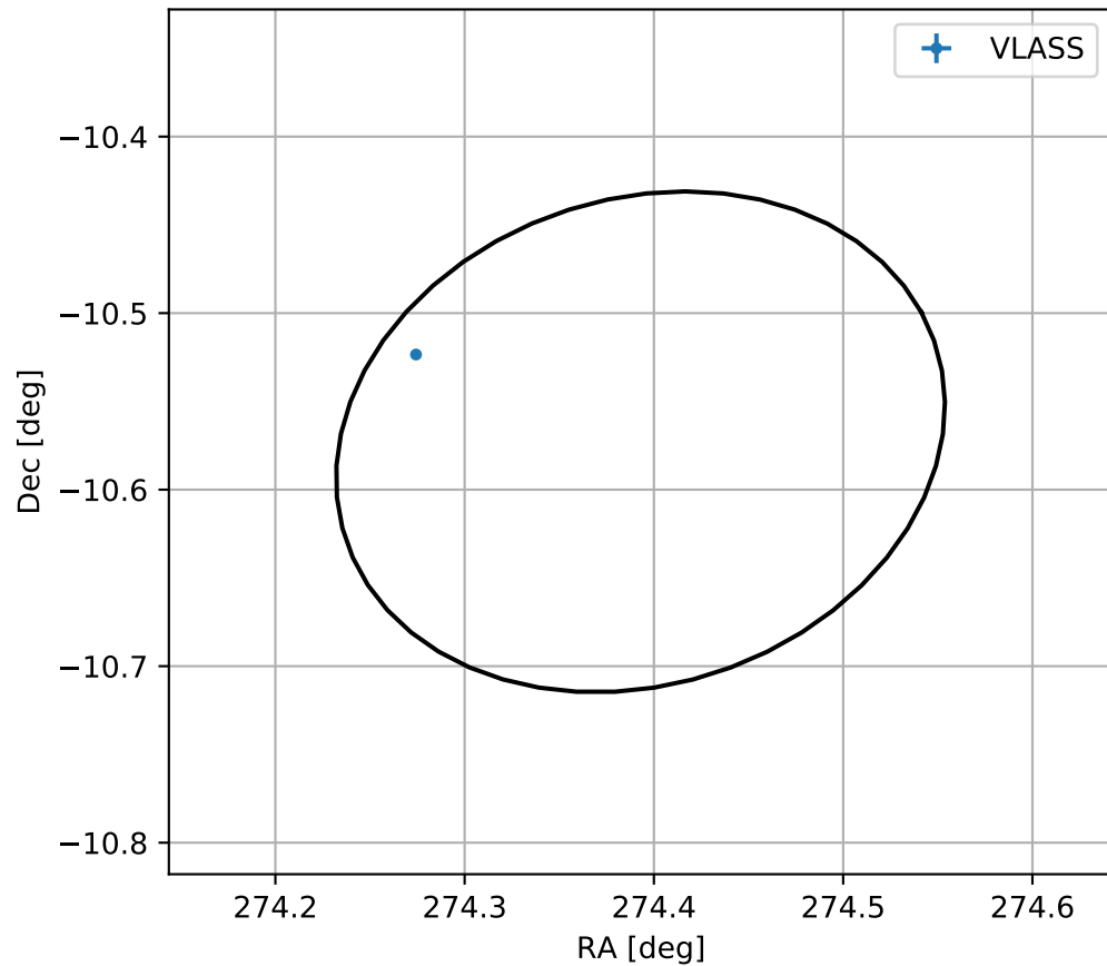
4FGL J1817.5-1034
