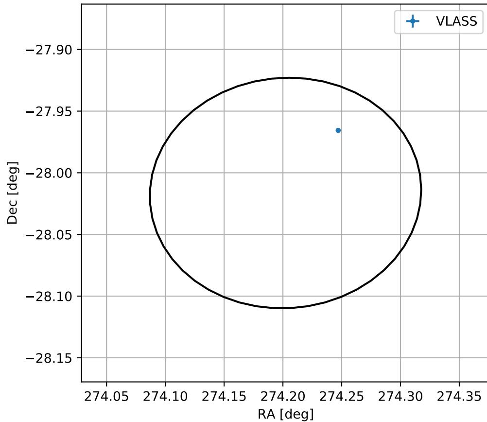
4FGL J1816.8-2800
