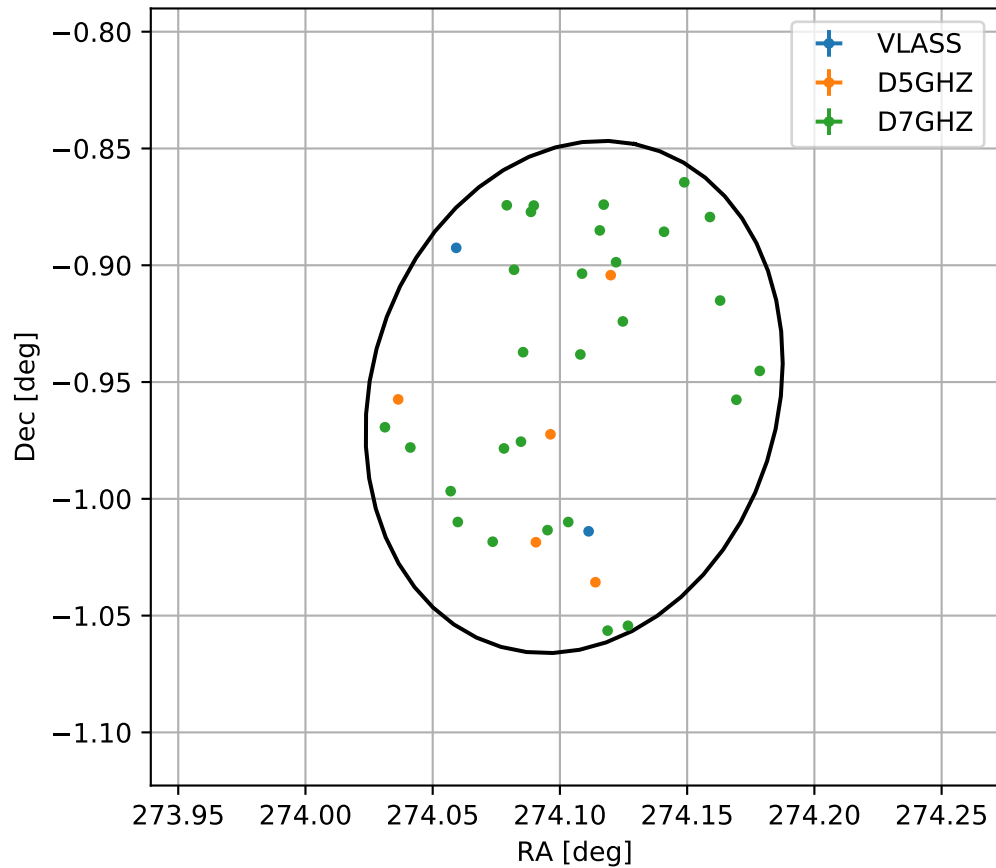
4FGL J1816.4-0057
