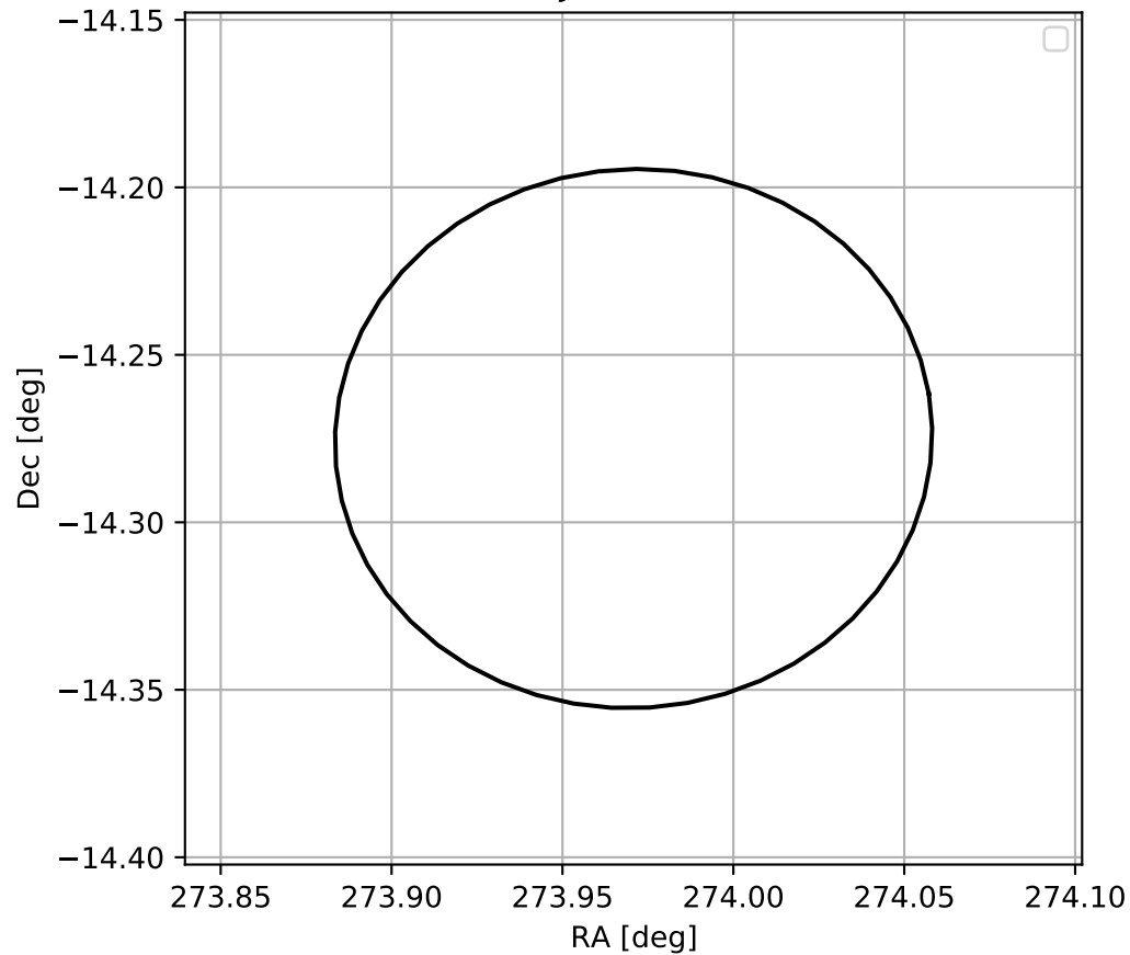
4FGL J1815.8-1416
