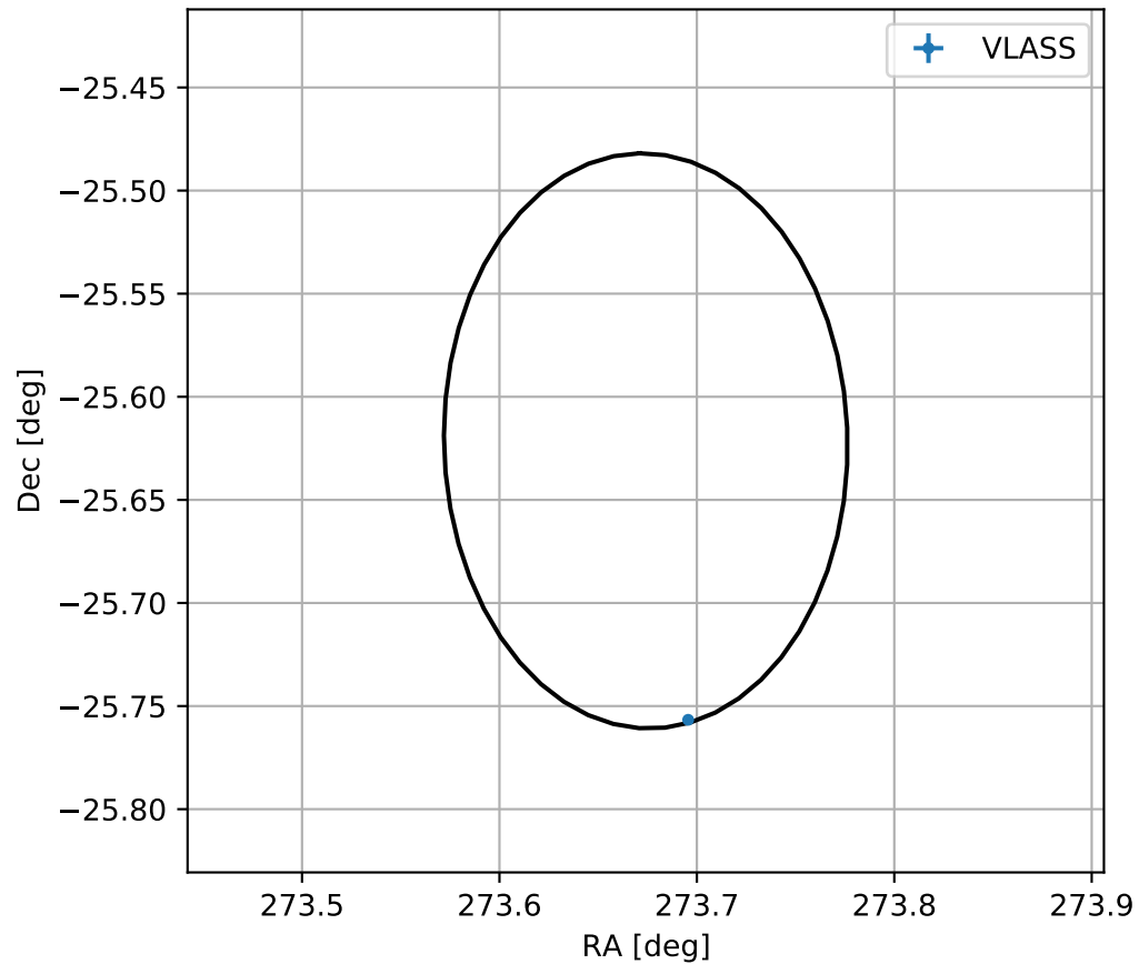
4FGL J1814.6-2537
