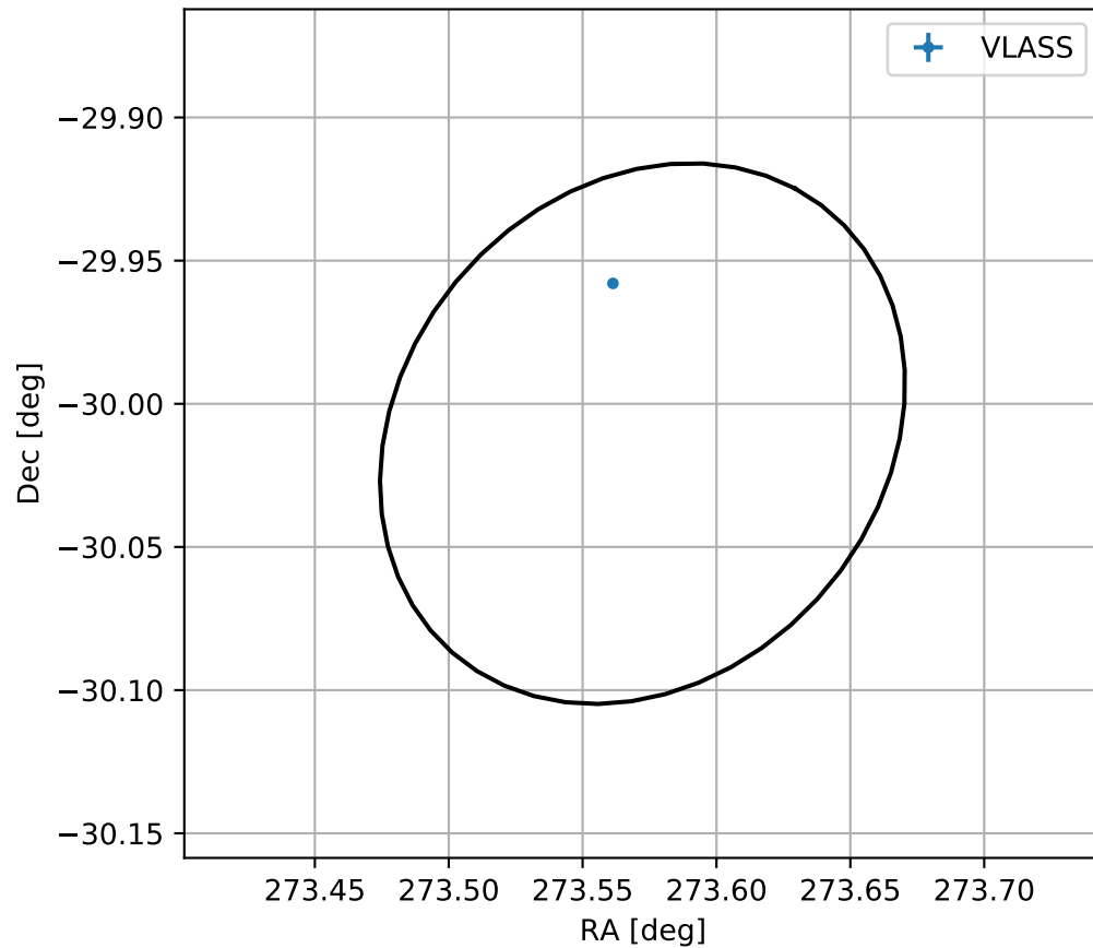
4FGL J1814.2-3000
