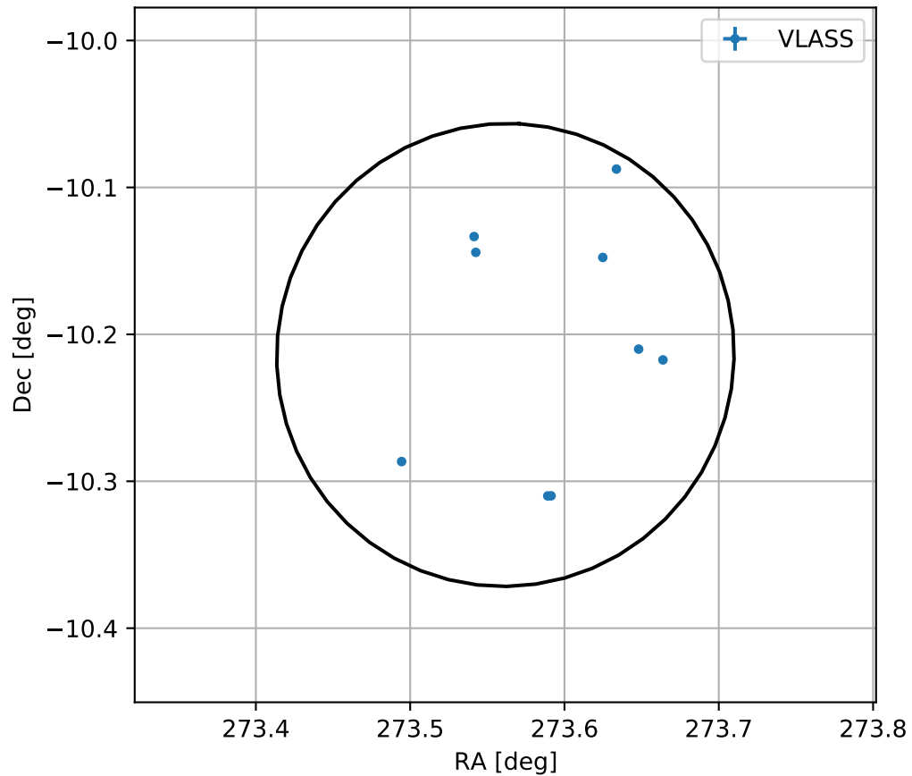
4FGL J1814.2-1012
