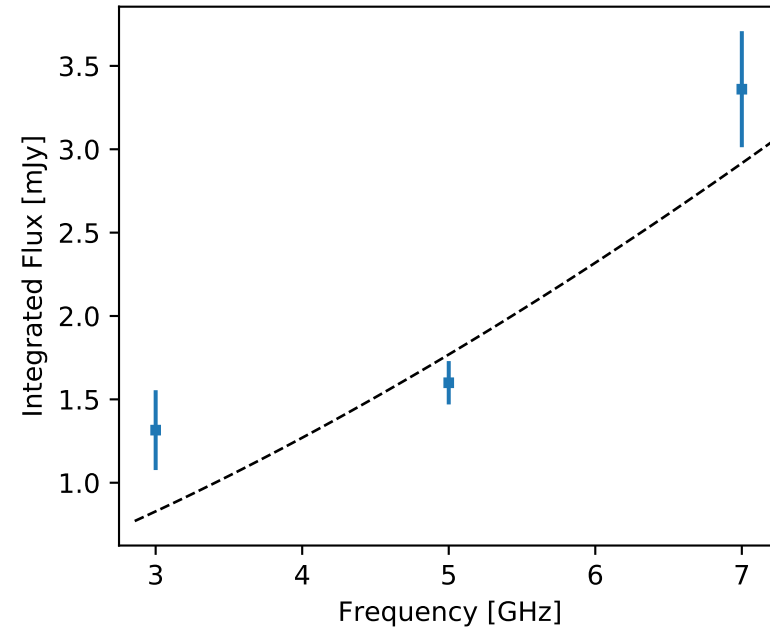
F357 J181340.36-115049.1 (unr)
