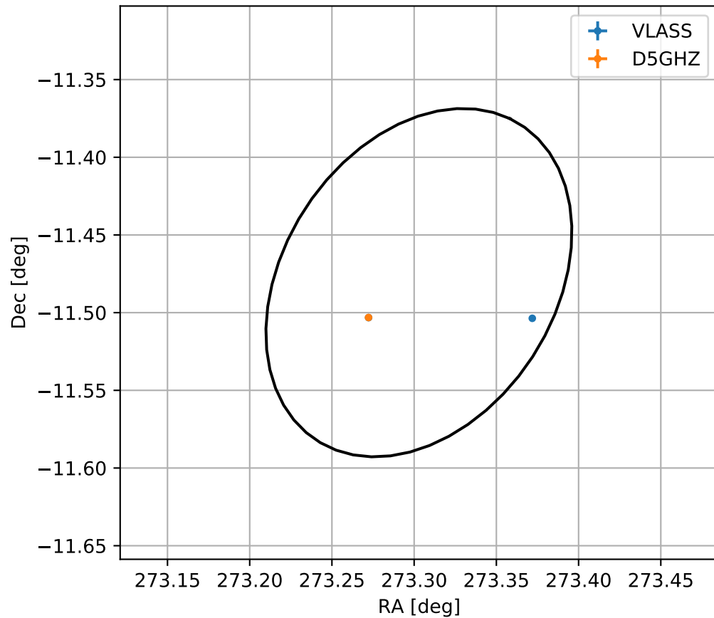
4FGL J1813.2-1128
