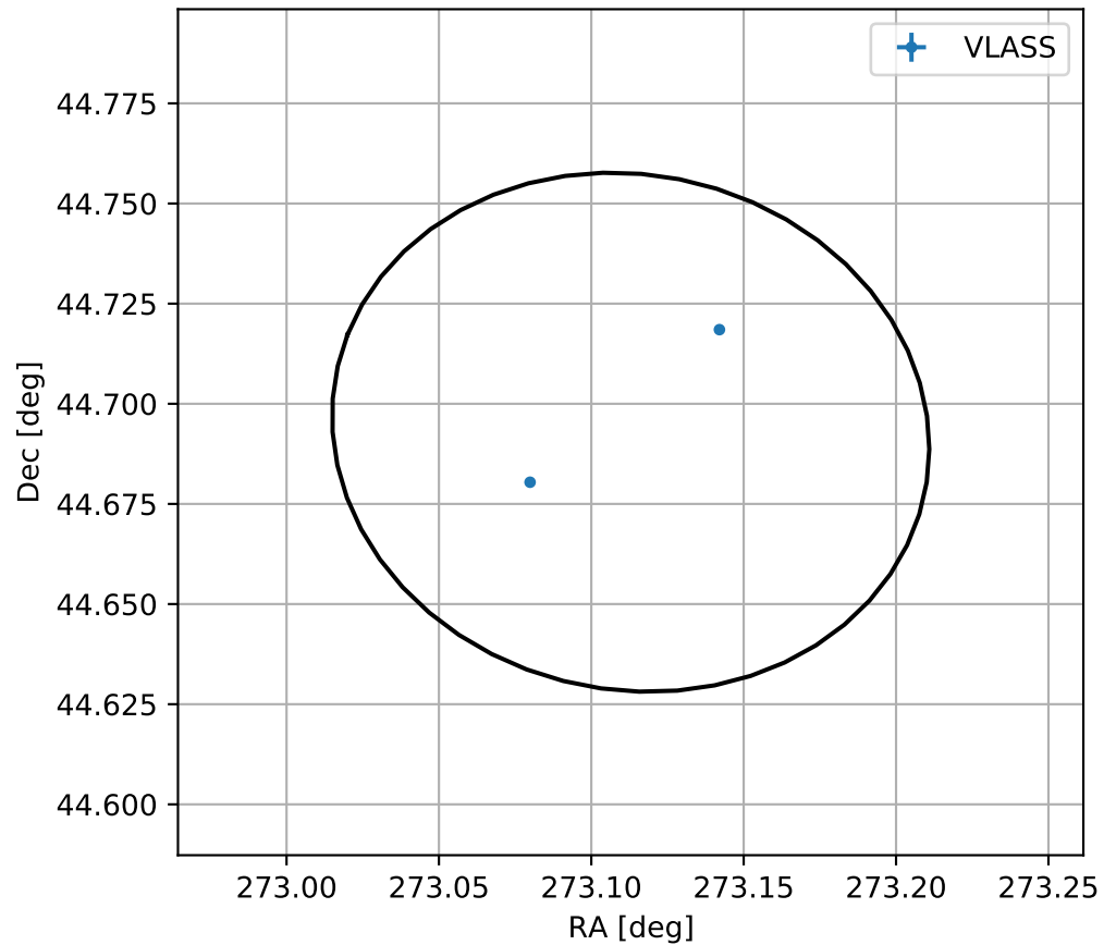
4FGL J1812.4+4441
