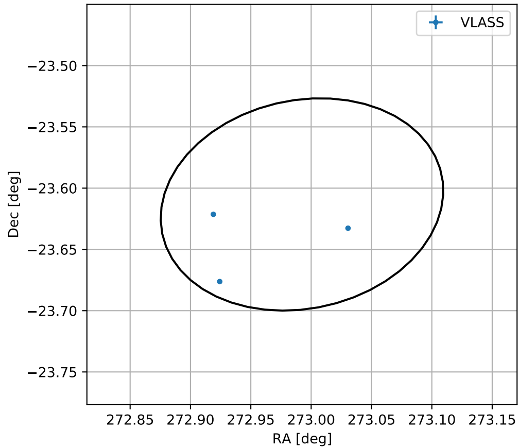
4FGL J1811.9-2336
