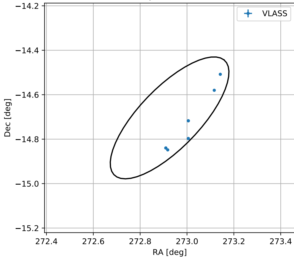
4FGL J1811.7-1442
