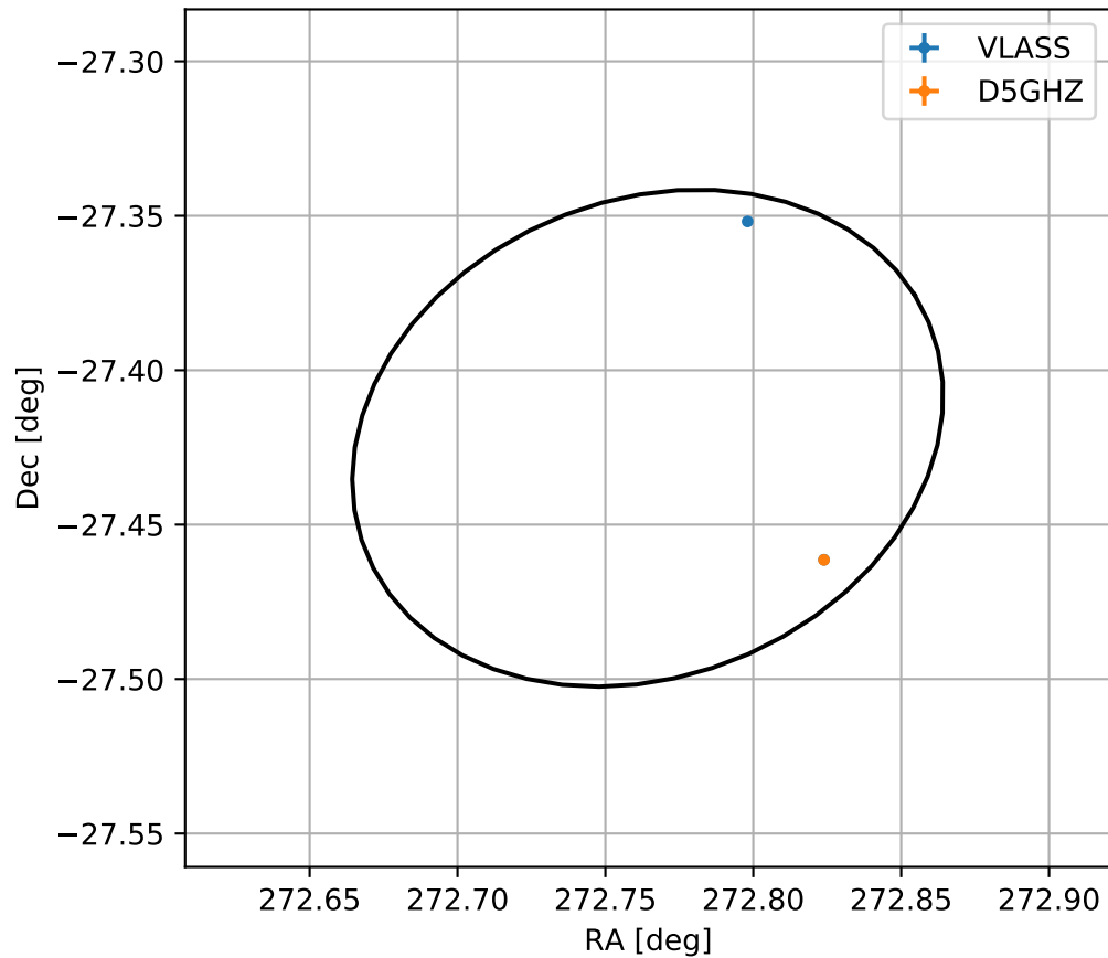
4FGL J1811.0-2725
