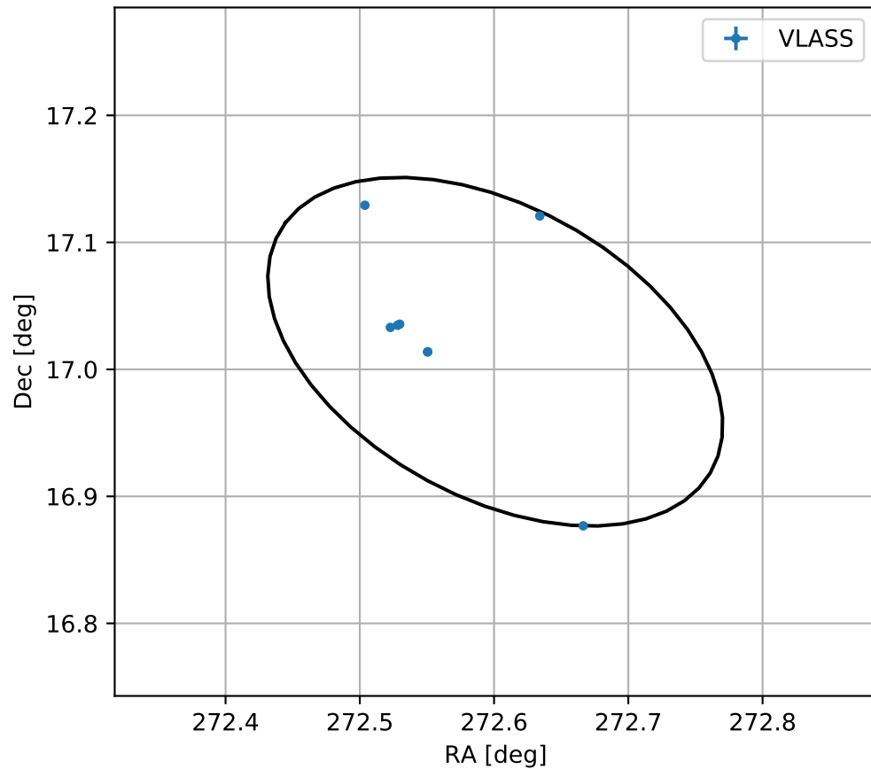
4FGL J1810.4+1700
