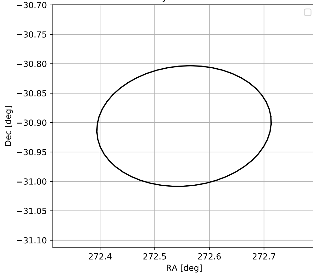
4FGL J1810.2-3054
