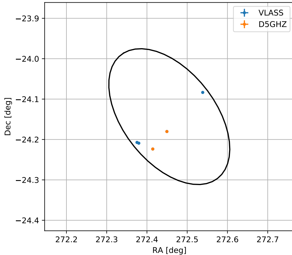
4FGL J1809.8-2408c
