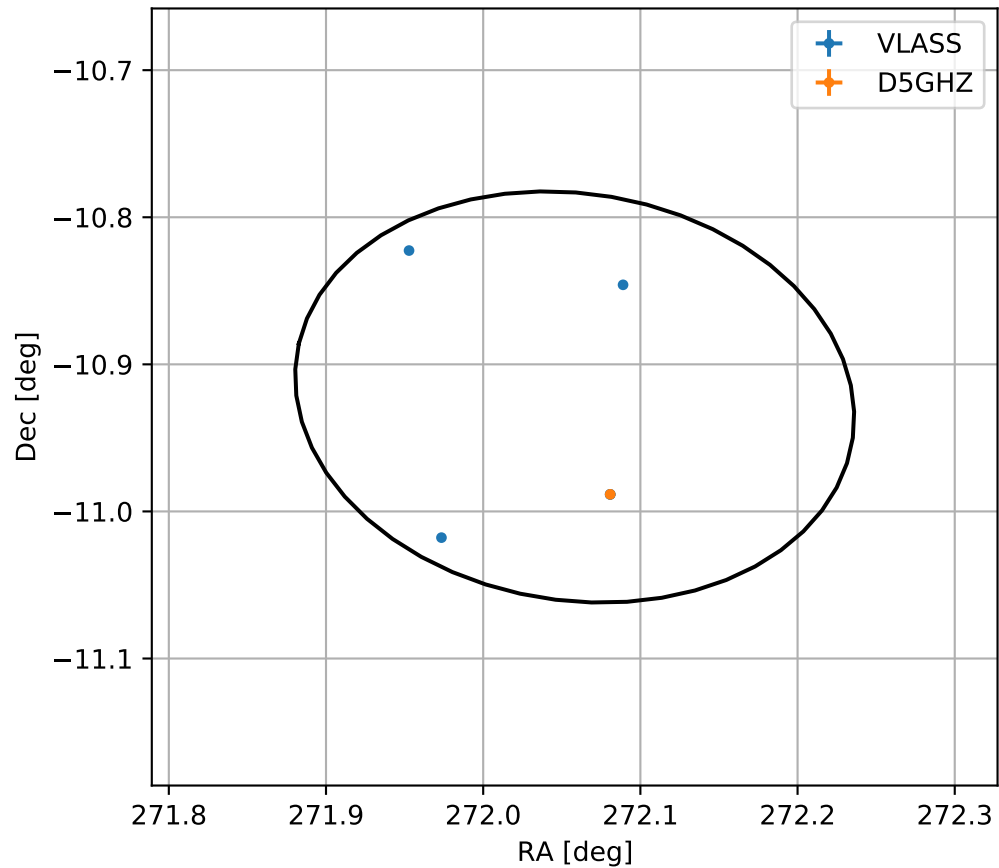
4FGL J1808.2-1055
