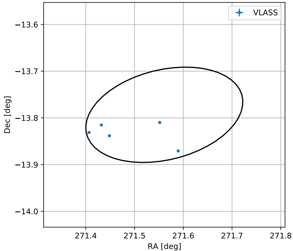
4FGL J1806.2-1347
