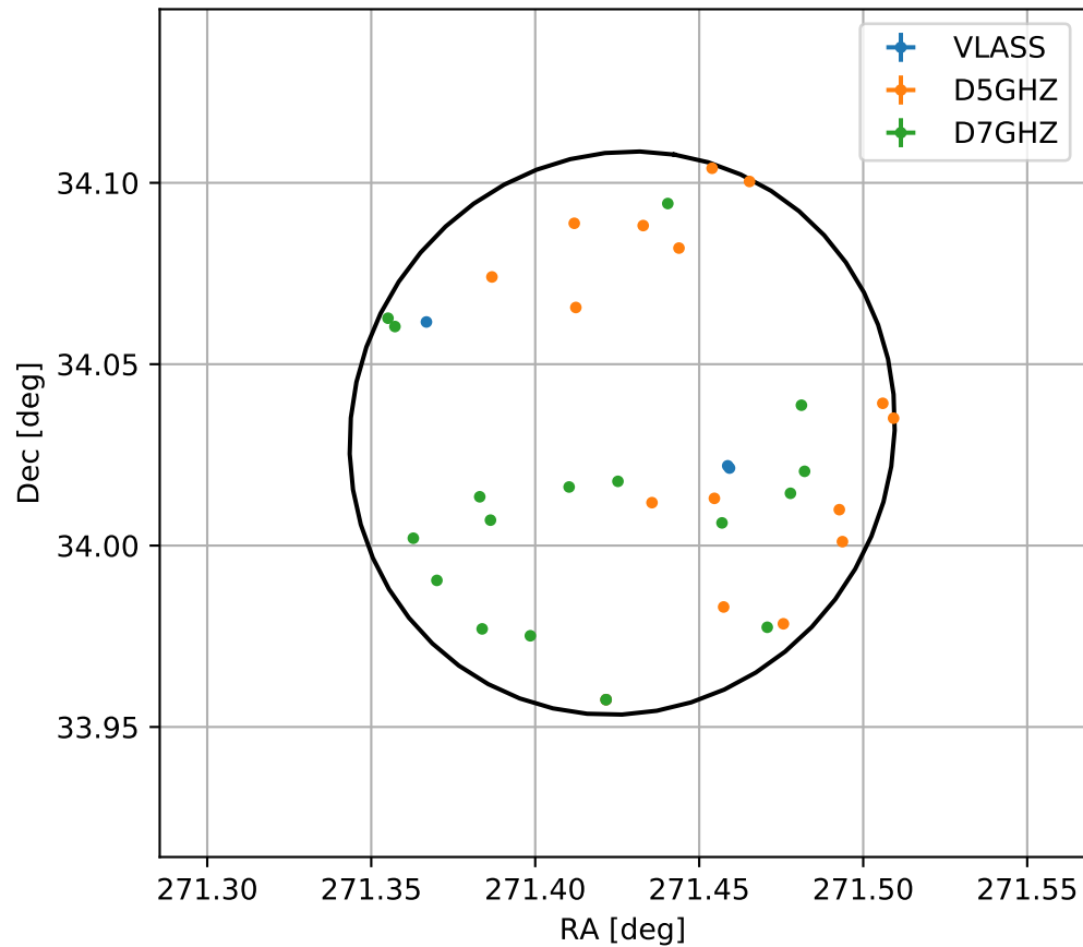
4FGL J1805.7+3401
