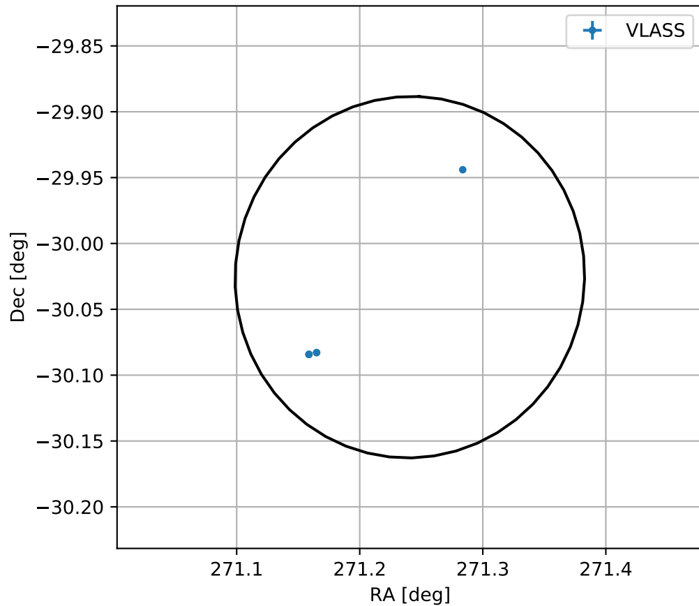
4FGL J1804.9-3001
