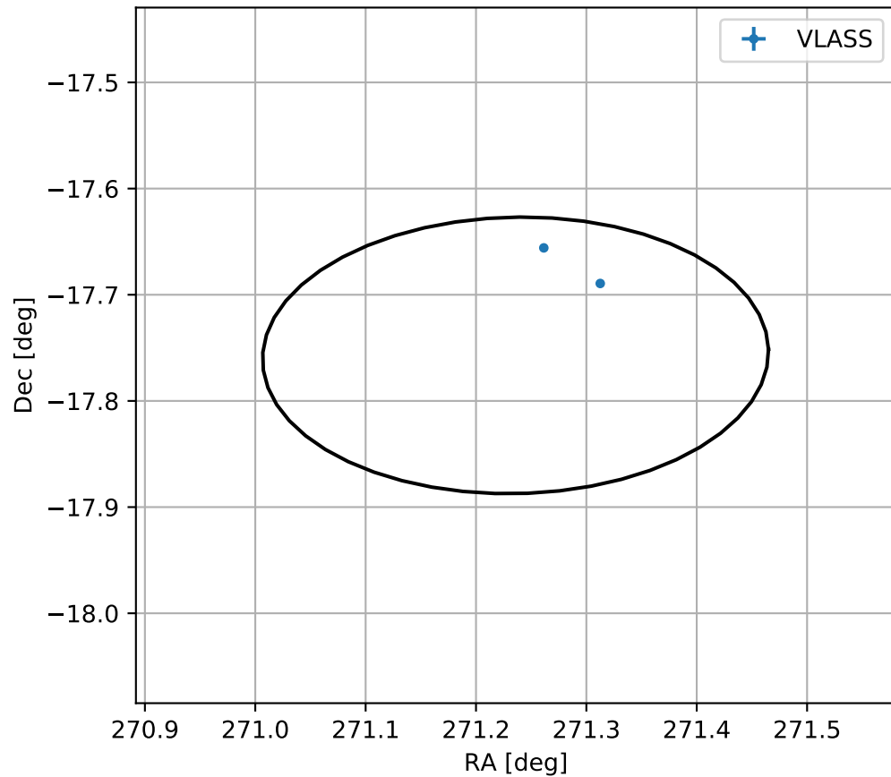
4FGL J1804.9-1745
