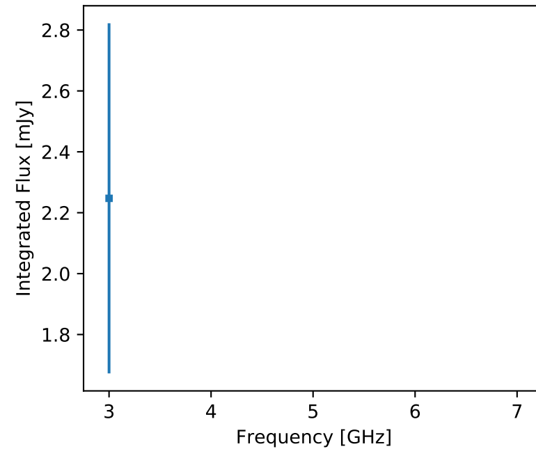
F357 J180515.01-174121.7 (unr)
