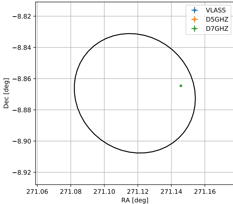
4FGL J1804.4-0852
