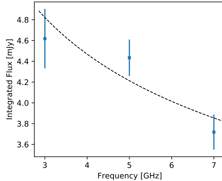
F357 J180434.96-085152.5 (unr)
