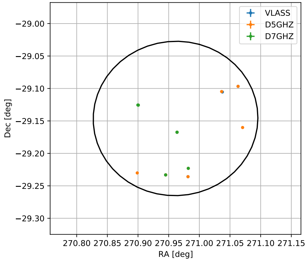
4FGL J1803.8-2908
