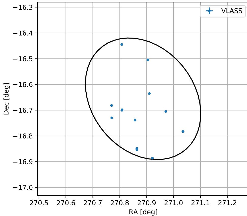
4FGL J1803.5-1639
