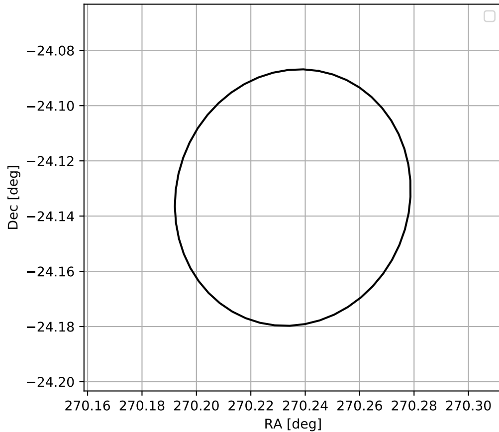
4FGL J1800.9-2407
