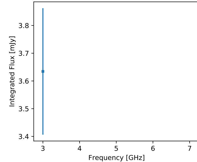
F357 J180031.34-290719.5 (unr)
