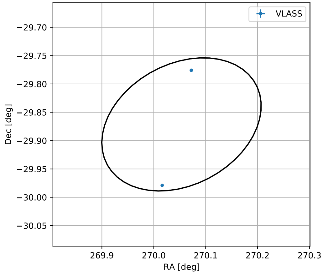
4FGL J1800.2-2952
