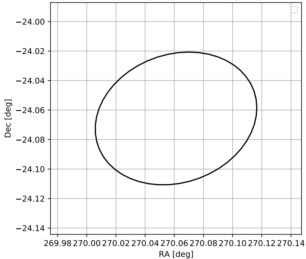
4FGL J1800.2-2403c
