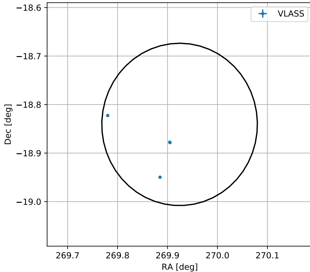
4FGL J1759.6-1850
