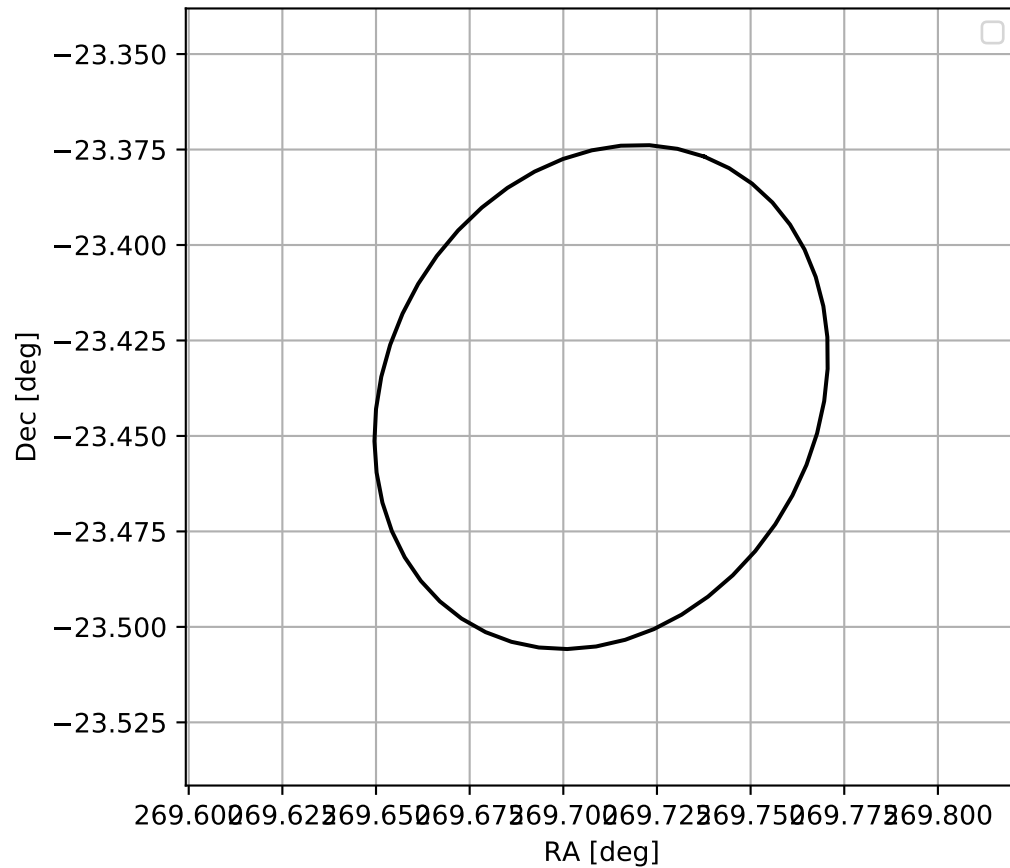
4FGL J1758.8-2326
