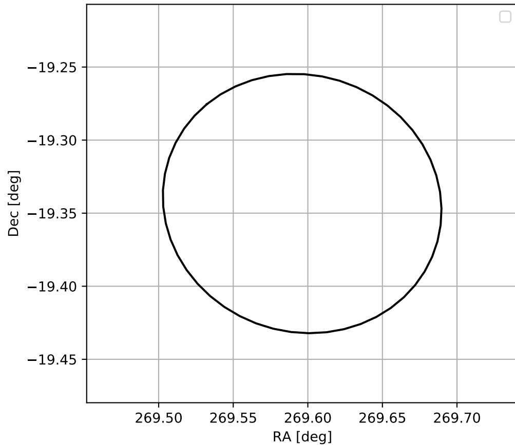
4FGL J1758.3-1920
