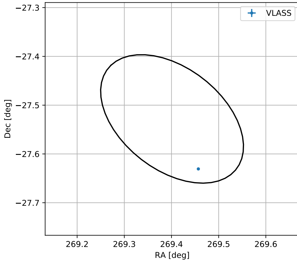
4FGL J1757.6-2731
