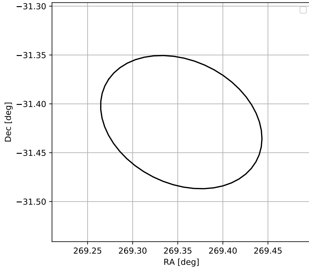
4FGL J1757.4-3125
