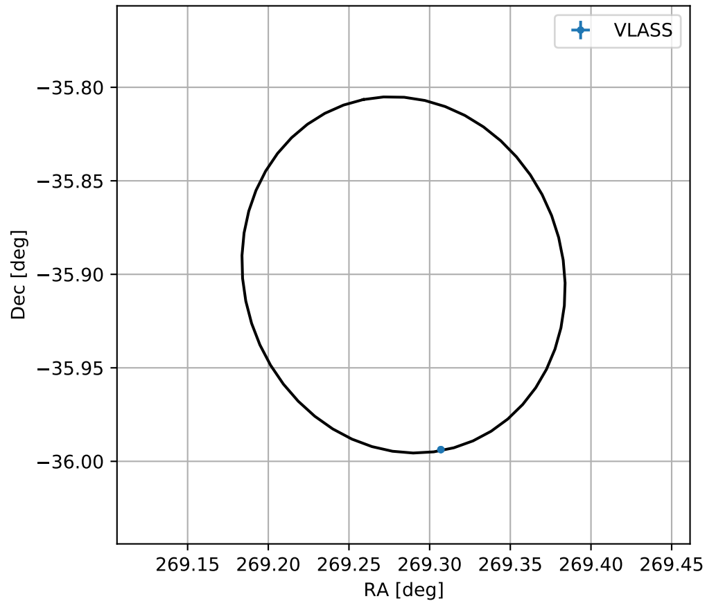
4FGL J1757.1-3554
