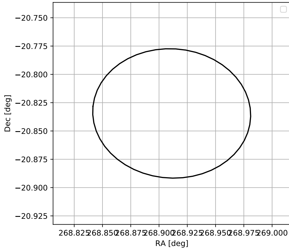
4FGL J1755.6-2050
