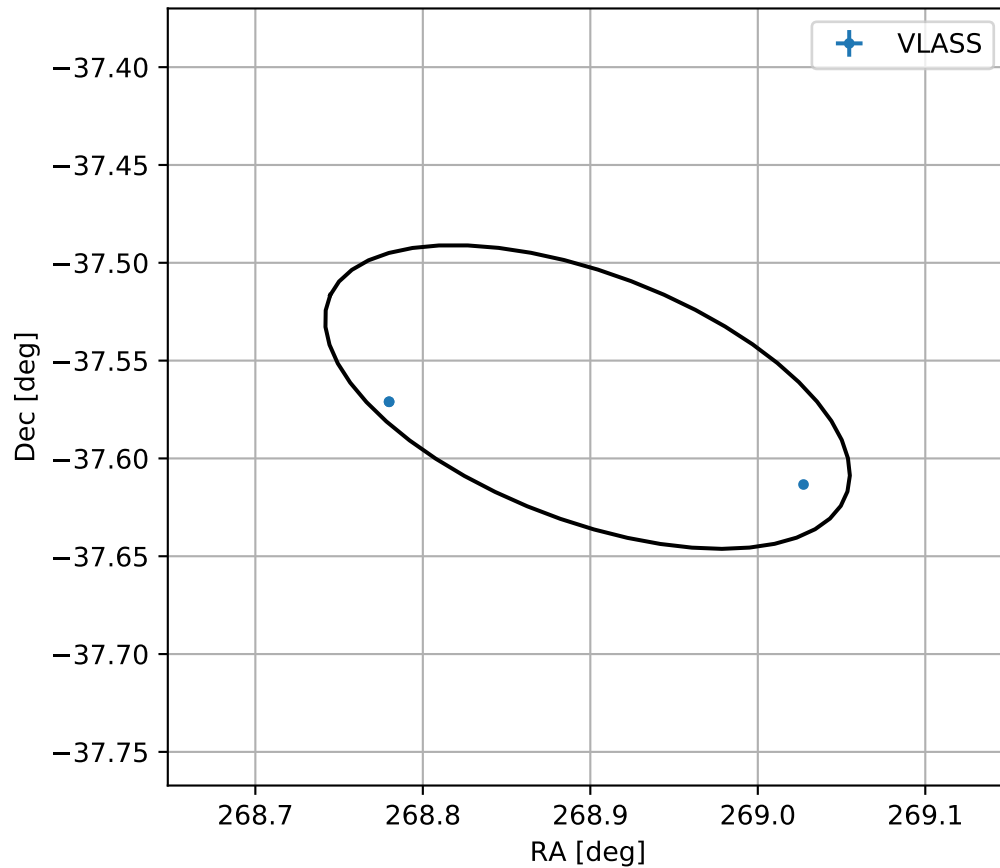
4FGL J1755.5-3734
