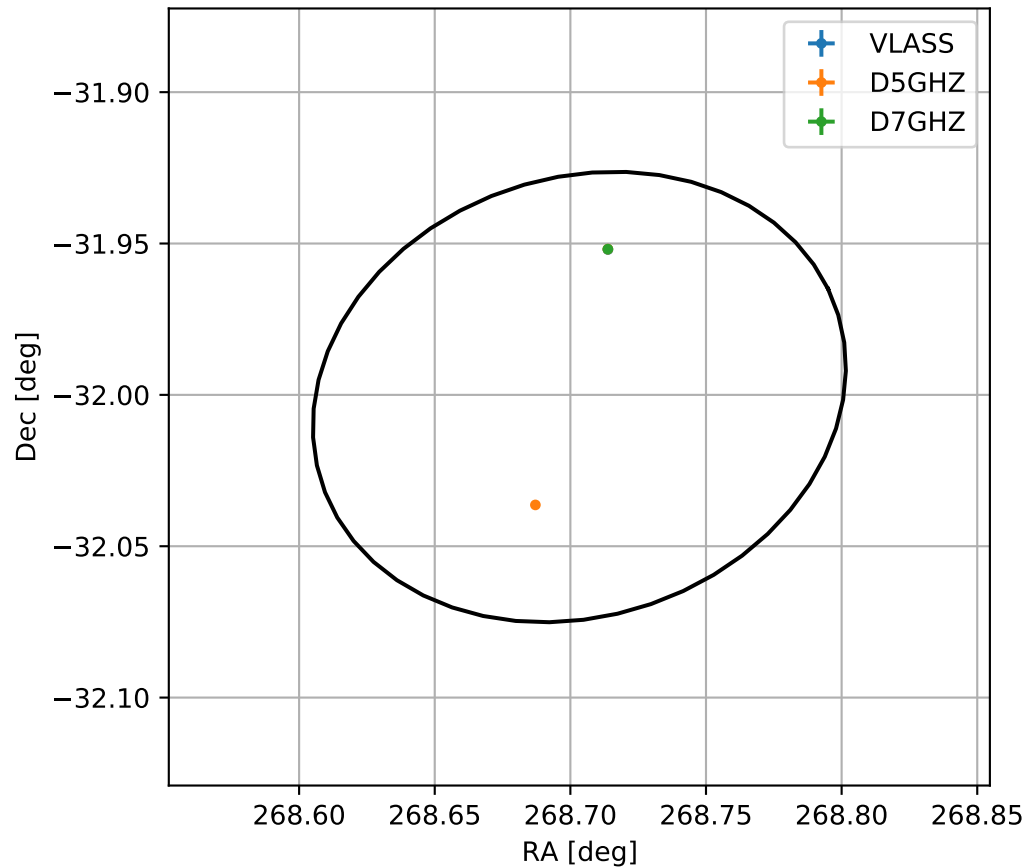
4FGL J1754.8-3200
