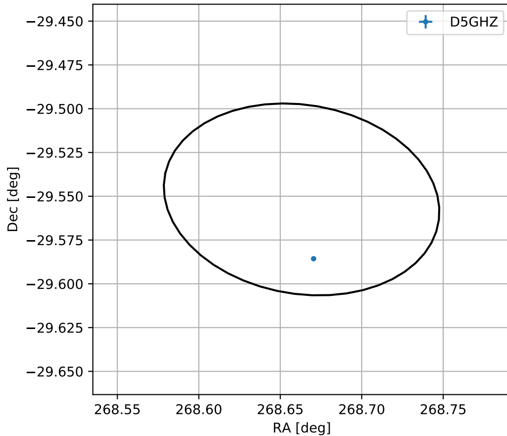
4FGL J1754.6-2933
