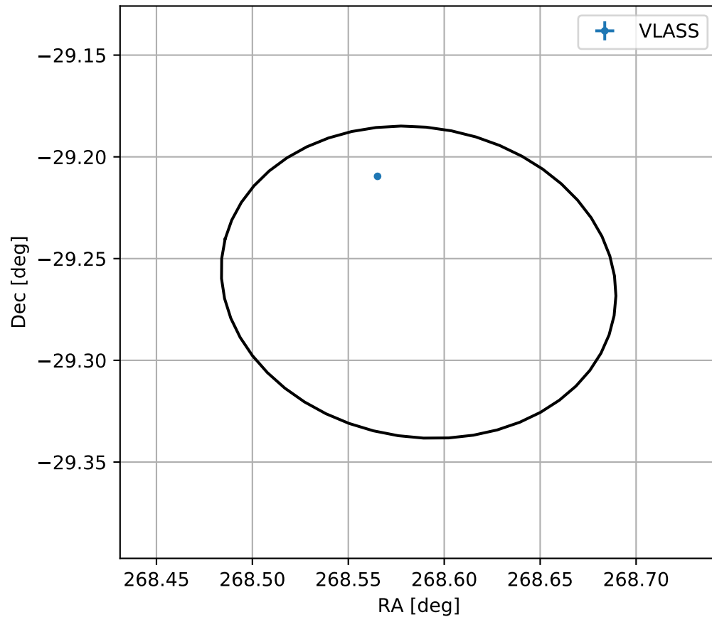
4FGL J1754.3-2915
