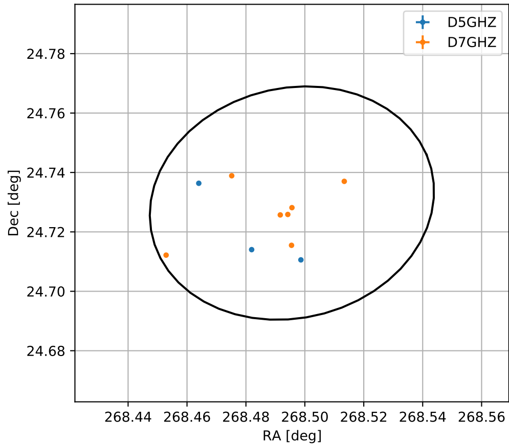
4FGL J1753.9+2443
