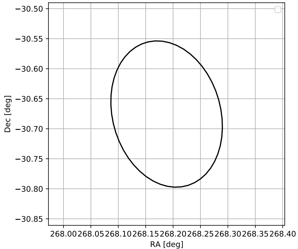
4FGL J1752.7-3040
