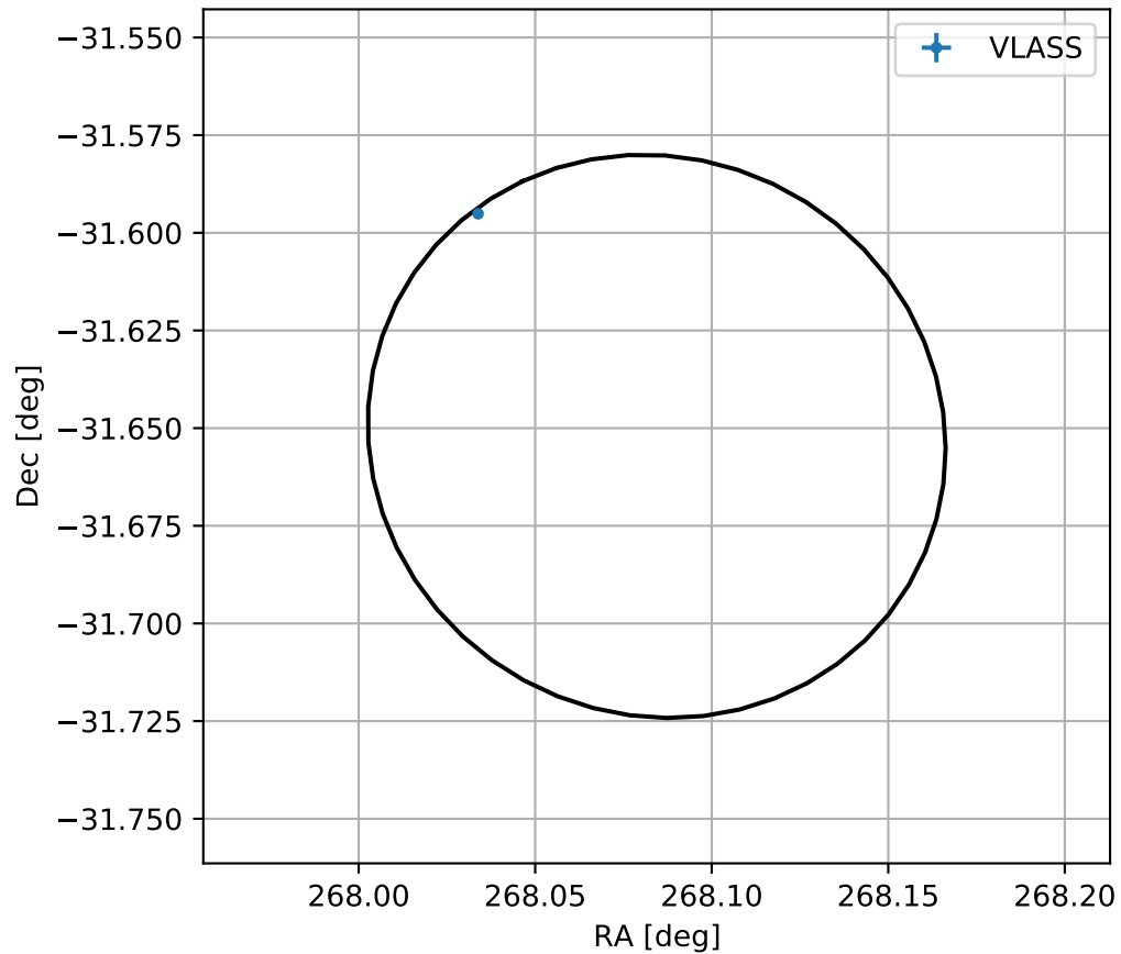
4FGL J1752.3-3139
