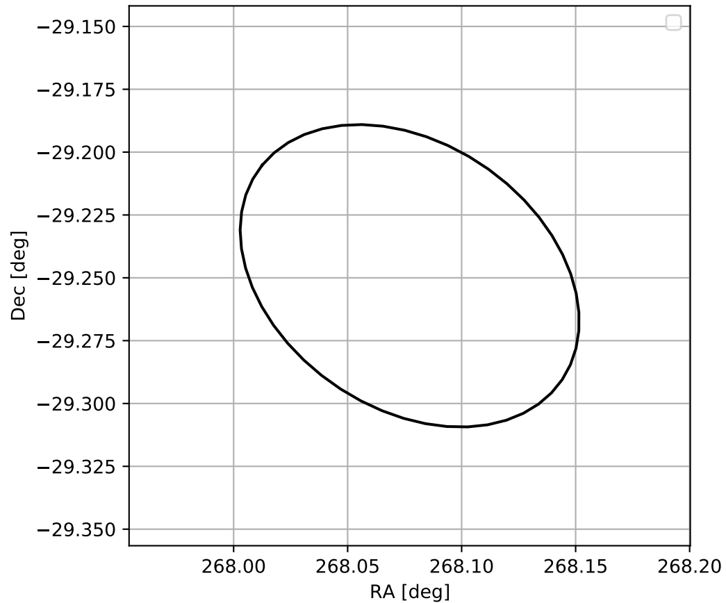
4FGL J1752.3-2914
