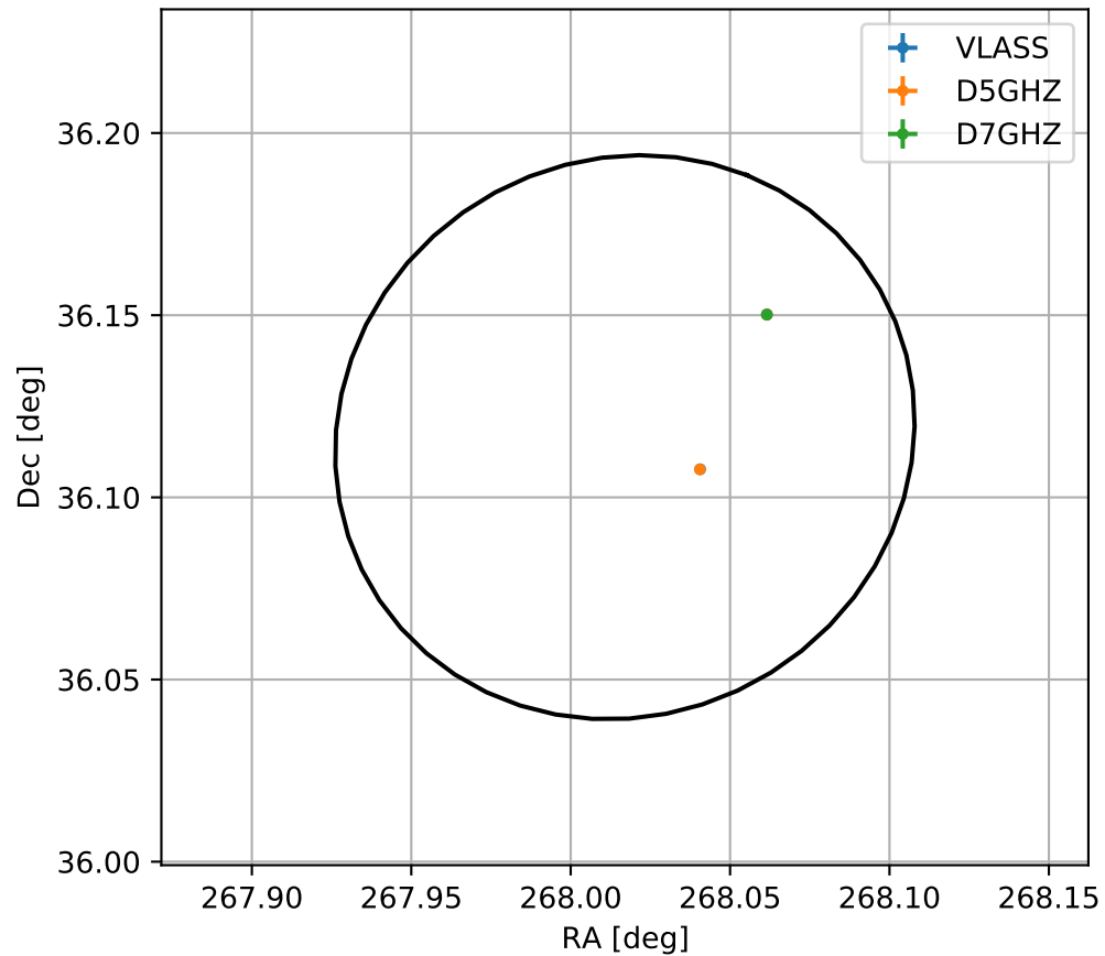
4FGL J1752.0+3606
