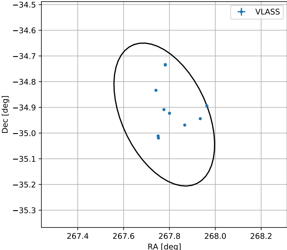
4FGL J1751.1-3455
