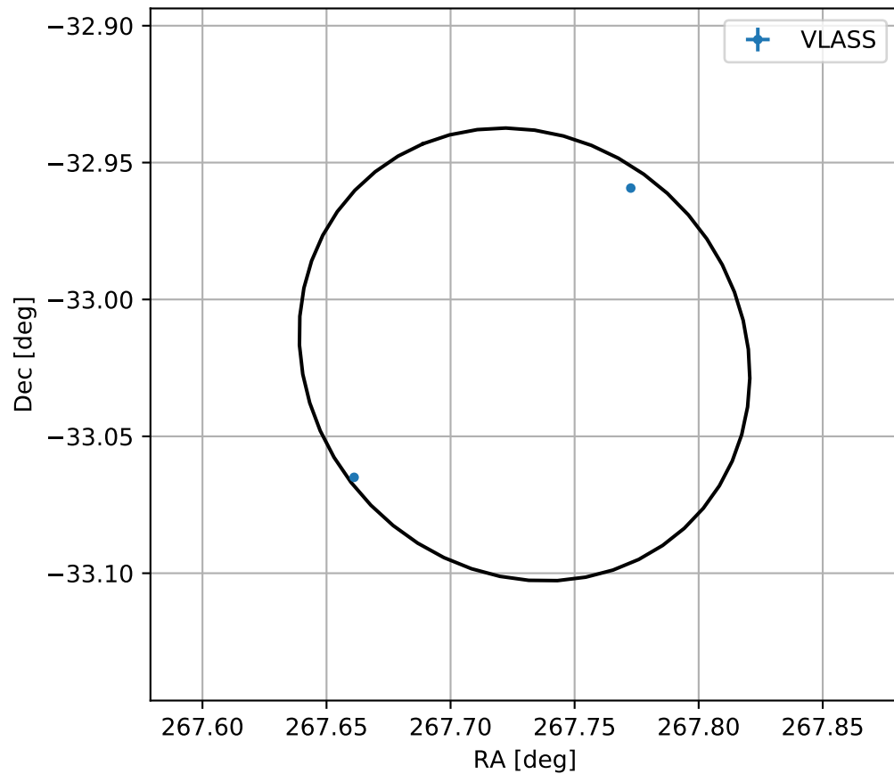
4FGL J1750.9-3301
