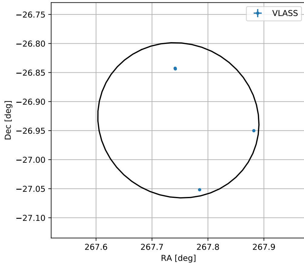
4FGL J1750.9-2655
